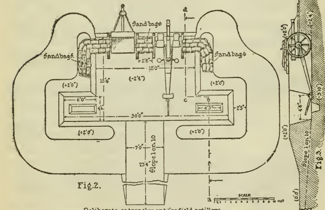
Deliberate entrenchment for field artillery. Suitable type when depression is necessary for concealment
